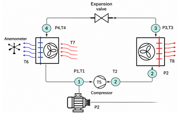
Figure 3. Sensors installed in the experimental test bench.
