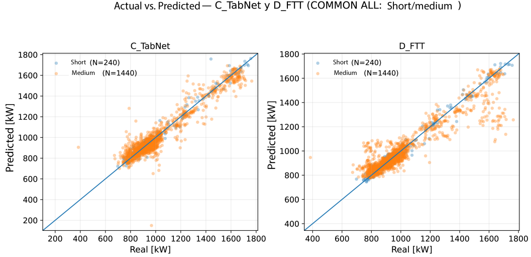
Figure 5. Observed vs. predicted values for C_TabNet and D_FTT across both forecasting horizons (rolling-origin; COMMON ALL). The line indicates y = x .
