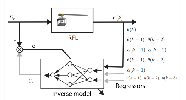
Figure 1. Scheme of the RFL inverse dynamics identification process.
