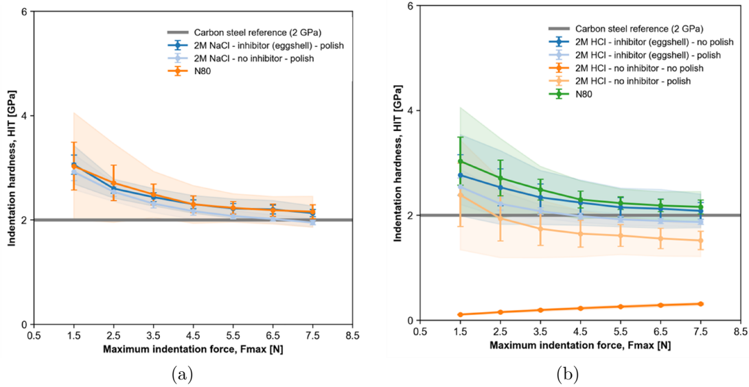
Figure 3. Indentation hardness. a) Brine - 2 M NaCl; b) Acid - 2 M HCl. Note: shaded area shows \pm 1 standard deviation, bars show \pm 1 standard error, and data points show mean values.
