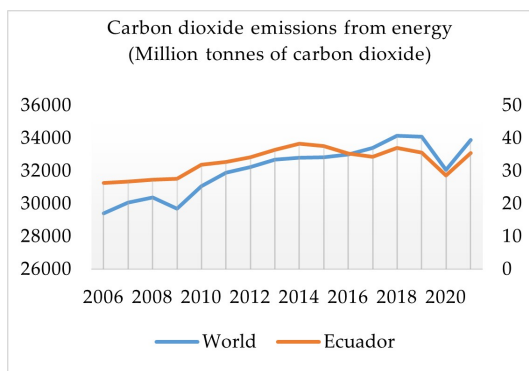
Figure 1. CO_2 emissions (2007 – 2021)
