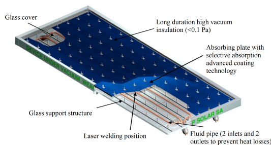
Figure 5. Structure of the evacuated flat plate collector [25]
